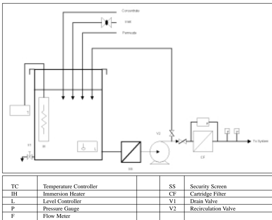
Figure 2 Cleaning Equipment
